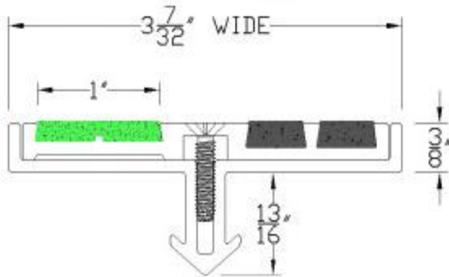
3 7/32" wide, 3/8" thick DRAWING NOT TO SCALE
